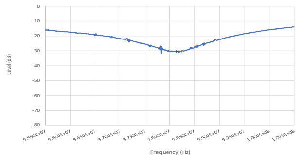
Return loss
